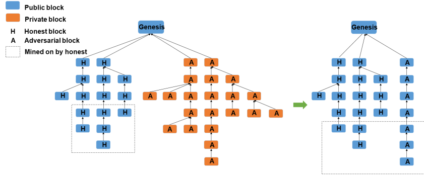
Fig. 5: Private attack on g -greedy protocol with g = 2
