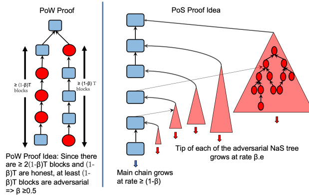
Fig. 1: Left: In the PoW case, a counting argument shows that since (1 - \beta) blocks are adversarial, the adversary power \beta \geq (1 - \beta) . This proof fails to work in the PoS case. Right: Our proof technique. Race between main chain and adversarial trees: adversary-proof convergence happens at a honest block if none of the previous NaS trees can ever catch up with the main chain downstream of the honest block. Security is proven by showing these events occur often.
