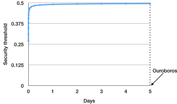
Fig. 2: The security threshold \beta_c^* of c -Nakamoto-PoS against the prediction window, equaling to c times the inter-block time, which we set to be 20s, to match the implementation of Ouroboros in Cardano. The Cardano project currently updates the common randomness every 5 days (21600 blocks, or 10\kappa ), while the security threshold of c -Nakamoto-PoS can approach 1/2 with much higher randomness update frequency.
